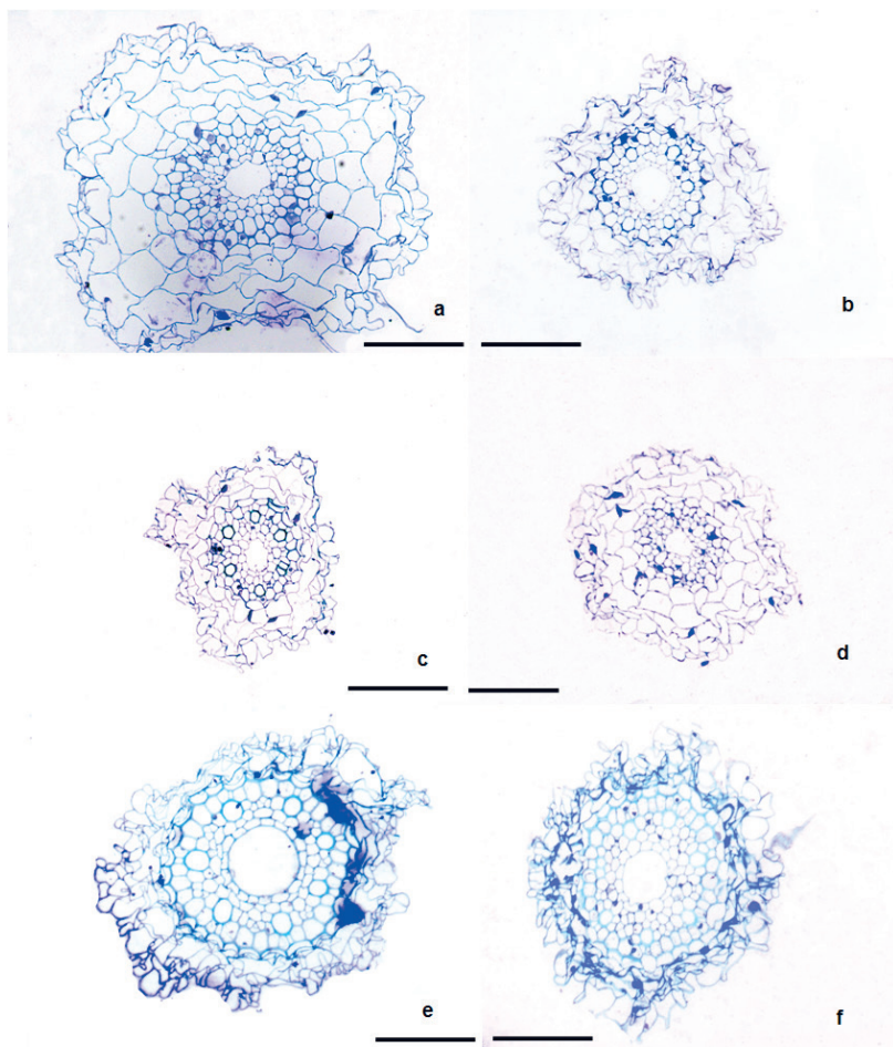
On-line Suppl. Fig. 1. Semi-thin cross section in control wheat root cells (a) and after 15 days of exposure to 0.5 (b), 1 (c), 5 (d), 10 (e), and 20 mg L -1 of AgNPs (f). Scale bars = 100 \mu m.
